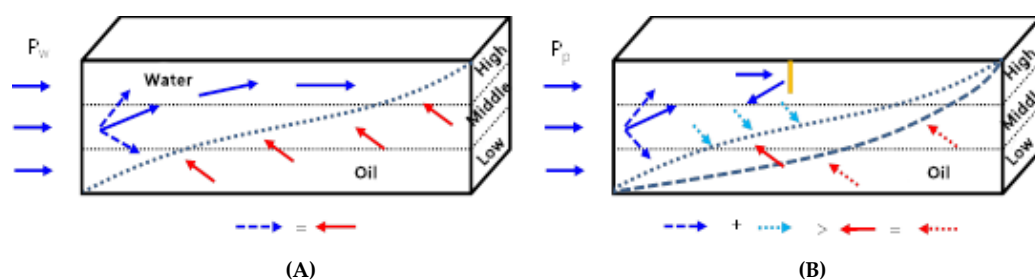
Figure 6. Schematic diagram of stress analysis before and after polymer injection. (A) is before injection, (B) is after injection).
